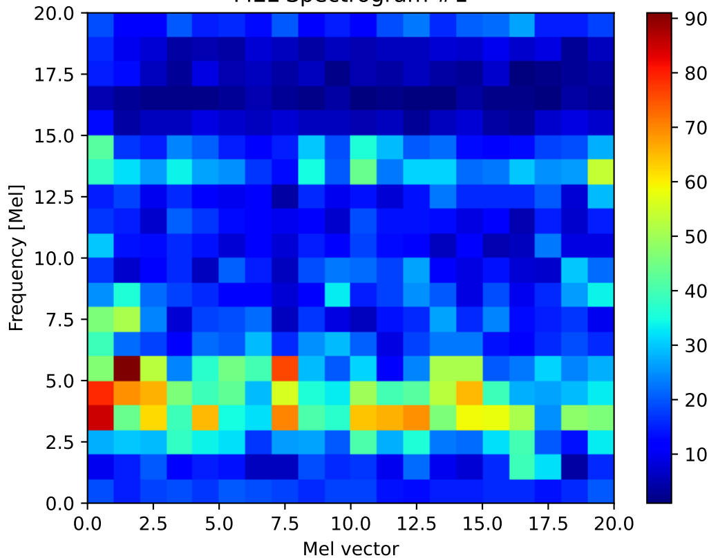
MEL Spectrogram #1
